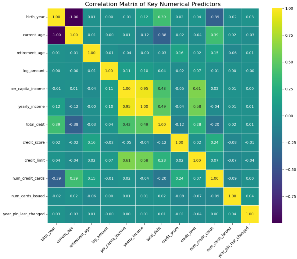
Figure 5: Numerical variable correlation heatmap
